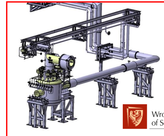
Cryogenic Distribution System
