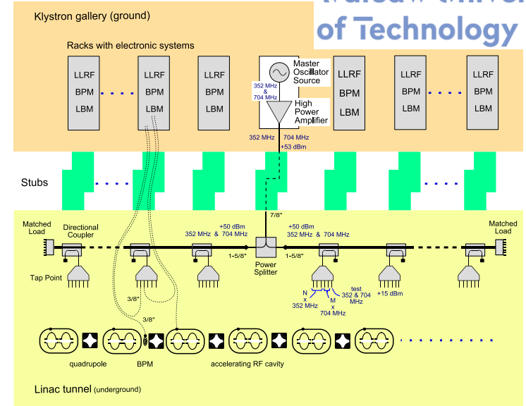
Phase Reference Line
