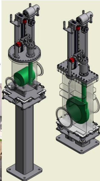
Gamma Blocker system
