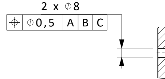
DETAIL C (1:2)
