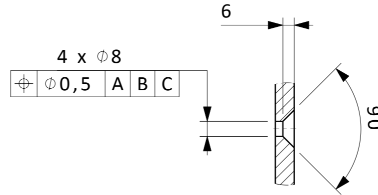
DETAIL B (1:2)
