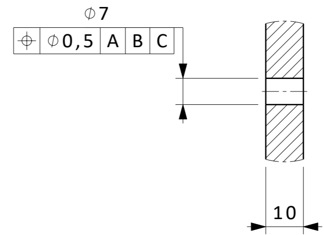
DETAIL B (1:1)
