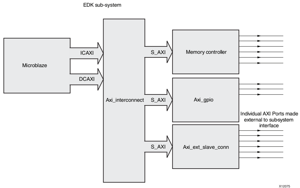
Figure 2-16: EDK Subsystem using an External Slave Connector
