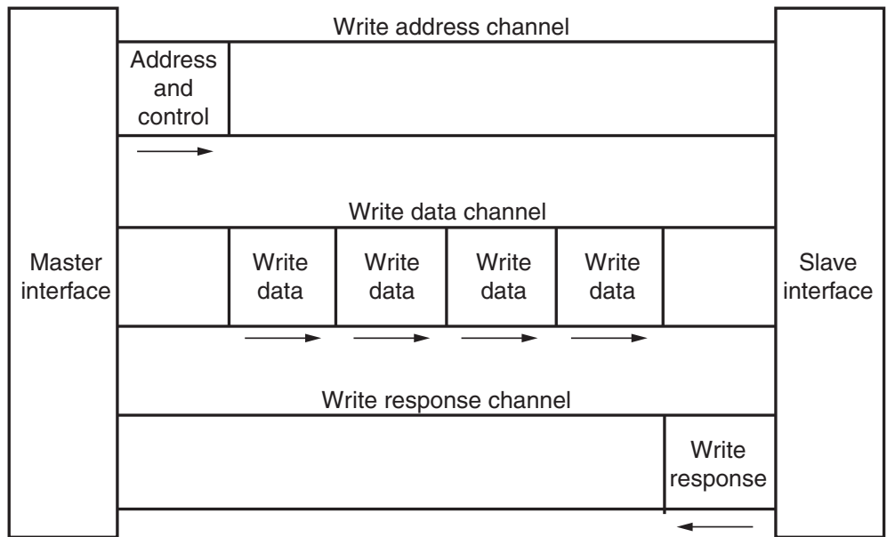
Figure 1-2: Channel Architecture of Writes
