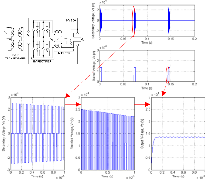
Fig. 5. Schematics of HV module and typical waveforms in pulsed mode
