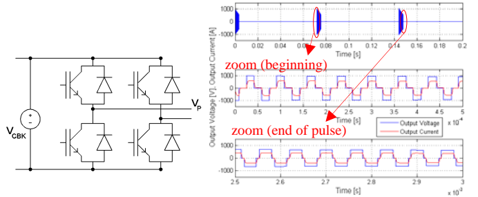
Fig. 4. Schematics of DC/AC H-bridge inverter and typical waveforms in pulsed mode
