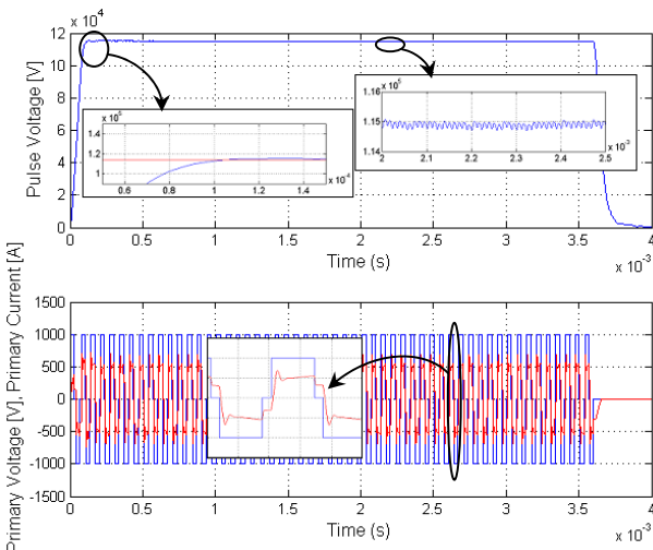
Fig. 13. Output pulse waveforms (simulation)
