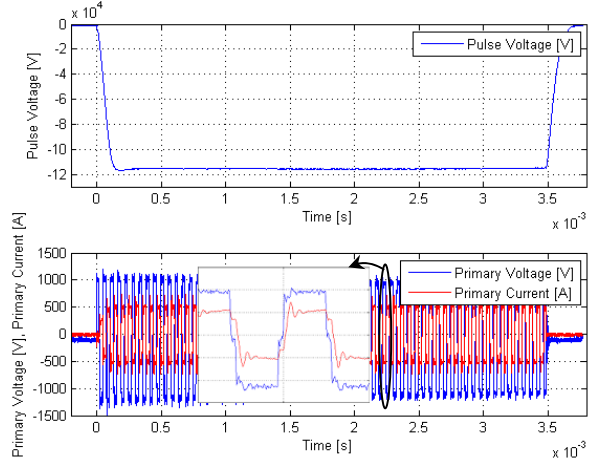
Fig. 15. Output pulse waveforms (experimental)
