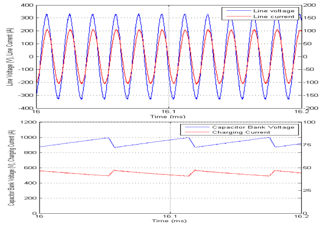
Fig. 14. Input side waveforms (experimental)
