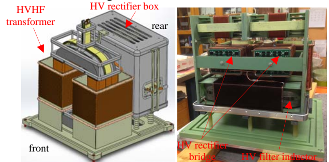
Fig. 11. One HV module; Left: 3D CAD model; Right: Picture from rear side without box enclosure
