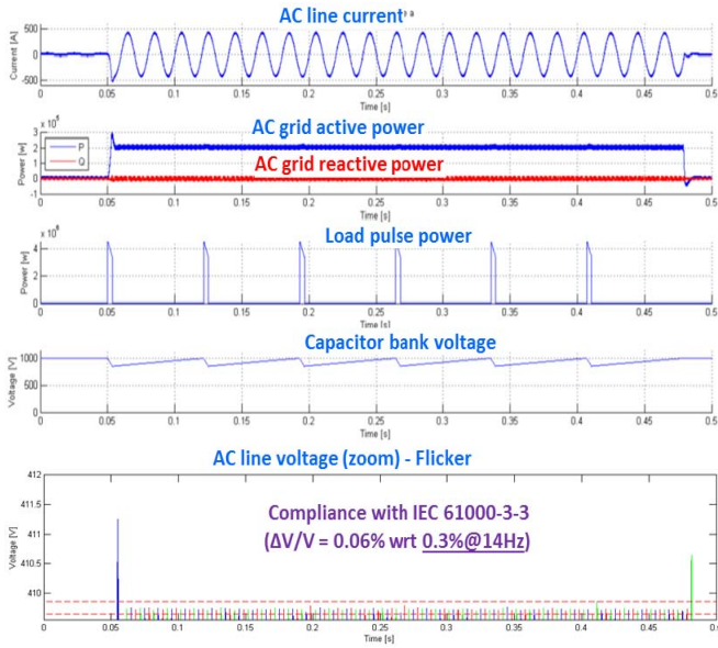
Fig. 12. Capacitor charger waveforms and AC grid power quality (simulation)
