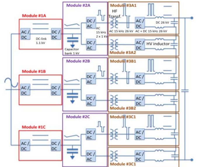
Fig. 6. SML modulator configuration diagram for ESS Linac
