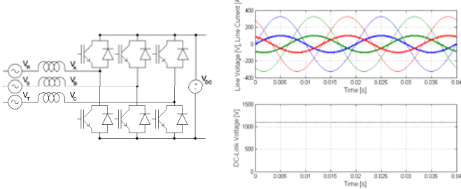
Fig. 2. Schematics of AC/DC Active Front End and typical waveforms
