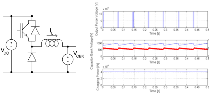
Fig. 3. Schematics of DC/DC Converter and typical waveforms
